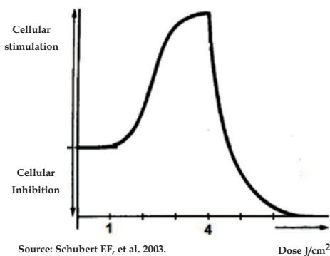
FIGURE 2: Arndt-Schultz Curve
