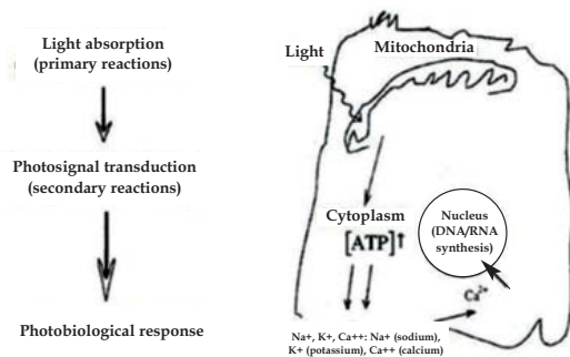
FIGURE 3: Karu Model
